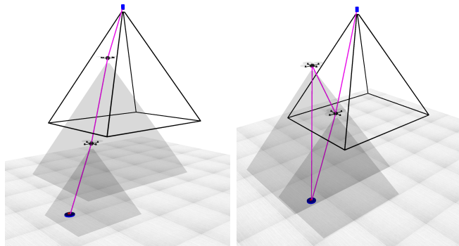
Fig. 10. An example of an advantage of our approach over the level-based approach. Left: most beneficial sensing topology for the level-based approach. The quadrotors form a chain topology as each level of quadrotors is allowed to sense only one level below it. Right: A superior sensing topology achieved by our novel method. The lower quadrotor is seen by the global sensor and the other quadrotor. The upper quadrotor can localize itself based on the observation of the lower quadrotor. Both quadrotors can observe the tracking target which provides more information than the level-based approach. There are no constraints for the topology levels.
