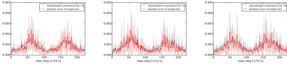
Fig. 4. Comparison of different time horizons in the optimization step. The time horizons are 2, 5, and 10, respectively. Evaluation measures are shown with 95% confidence intervals over 10 runs with 3 quadrotors. There is no significant difference in the tracking error for these time horizons.
