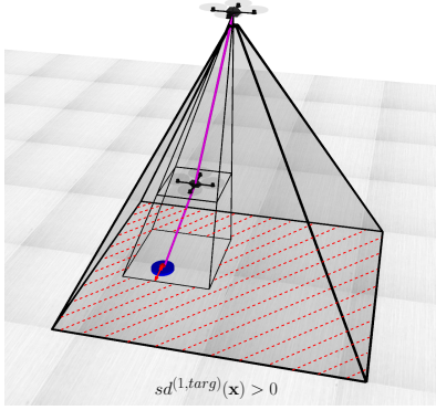
Fig. 3. Signed distance function in the presence of occlusions. First, we determine the shadows of all the occlusions such that the resulting field-of-view (the shaded area) is calculated. The signed distance is computed as the distance to the field-of-view.
