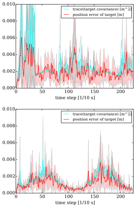
Fig. 8. Comparison between not taking occlusions into account in the optimization step (top) and accounting for occlusions using the signed distance function presented in this work (bottom). Statistics and 95% confidence intervals over 10 runs with 3 quadrotors. Taking occlusions into account is beneficial especially at the spots right below the global camera (i.e. start, middle and the end of the trajectory).
