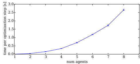
Fig. 7. Statistics over 10 runs of time per one optimization step for different number of quadrotors. Time per optimization step scales quadratically with the number of quadrotors.
