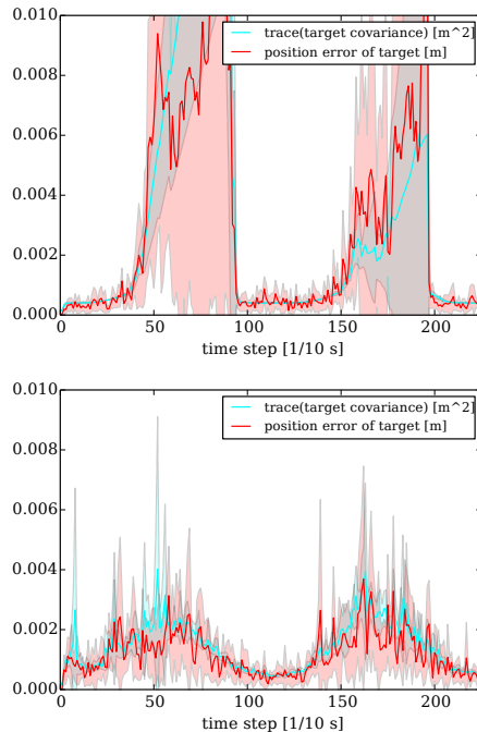
Fig. 9. Target tracking results for our previous level-based approach [12] (top) and the hereby presented method without explicitly reasoning about sensing topologies (bottom). Statistics and 95% confidence intervals over 10 runs with 3 quadrotors. The approach presented in this paper is more beneficial for the reasons explained in Fig. 10.
