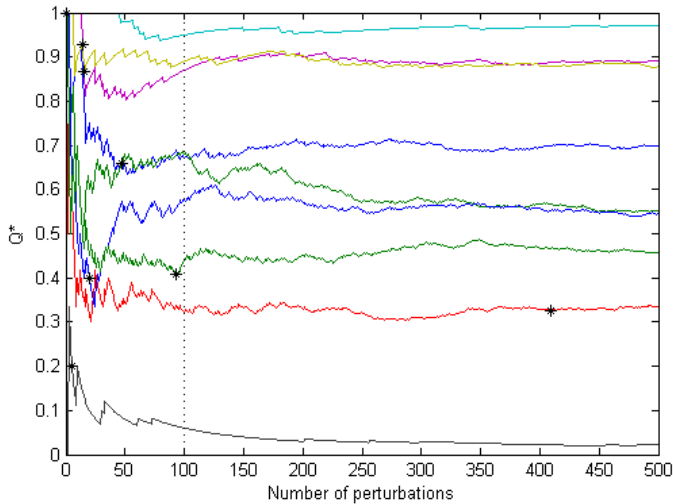
Fig. 9. Q^* vs. number of part perturbations evaluated for parts A-I in the test set. The point at which g^* stops changing is marked with an asterisk.
