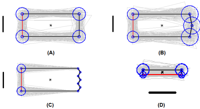
Fig. 10. Tolerancing results for selected parts. The best grasps on the highlighted edge were found with small tolerances shown as the smaller circles around the vertices with radius two standard deviations (95% confidence interval). The gripper width used for all parts is shown next to the part. Tests were performed as described in Section V-E using d_C = 0 , \rho = 4 , and |\Phi| = 5 , and for the indicated tests from that section, the tolerance for each vertex and center of mass is shown along with 100 perturbations of each part. Parts A and B are shown with tolerances that give comparable \hat{Q}^* (64.5 and 66.9, respectively), and suggest that friction closure is more sensitive to increased tolerances. Part D suggests that, relative to Part A, narrow parts have greater sensitivity to near-edge tolerances.
