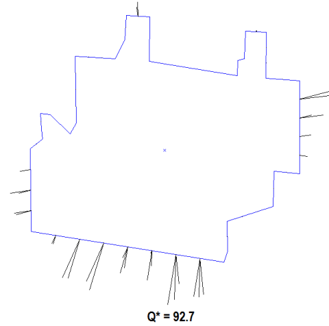
Fig. 7. “Whisker diagram” showing algorithm results for Part A, using d_C = 0 , \rho = 1.5 , and |\Phi| = 5 . Each line segment represents a candidate grasp, and indicates its nominal contact point on the part. The line segment indicates the approach lines for the grasp, and is orthogonal to the gripper jaw. The length indicating the Q -value relative to other segments. The approach line with the highest Q -value (i.e., the longest line segment) is labeled, and the jaw positions for this grasp is illustrated in Fig. 6.
