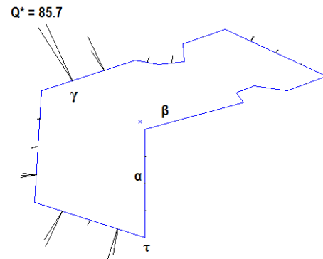
Fig. 8. “Whisker diagram” showing algorithm results for Part B, using d_C = 0 , \rho = 1.5 , and |\Phi| = 5 . The labels are used in Section V-A to illustrate various aspects of the results. Each line segment represents a candidate grasp, and indicates its nominal contact point on the part. The line segment indicates the approach lines for the grasp, and is orthogonal to the gripper jaw. The length indicating the Q -value relative to other segments. The approach line with the highest Q -value (i.e., the longest line segment) is labeled, and the jaw positions for this grasp is illustrated in Fig. 6.
