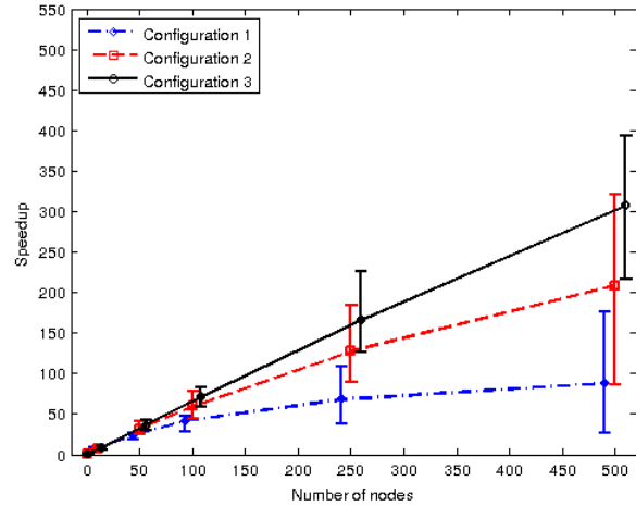
Fig. 16. Overall (i.e., worst case) MATLAB runtime speedup vs. number of nodes. The average, minimum, and maximum are shown for 1, 10, 50, 100, 250, and 500 nodes. The highest speedup is 393\times , for Part C with Configuration 3. The speedups are less than for the average times because with increasing numbers of nodes, the probability increases of a node taking significantly longer than average, increasing the overall (i.e., worst case) running time.
