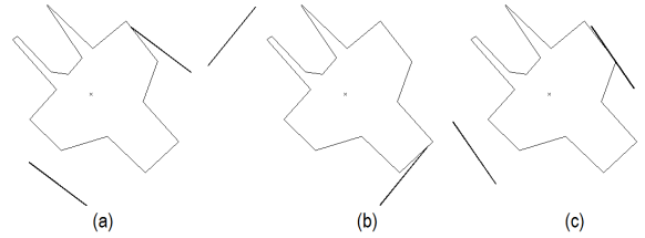
Fig. 19. Grasps tested for Object M.
