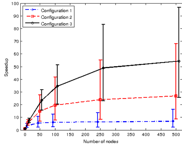
Fig. 17. Overall (i.e., worst case) PiCloud runtime speedup vs. number of nodes. The average, minimum, and maximum are shown for 1, 10, 50, 100, 250, and 500 nodes. The highest speedup is 97\times , for Part C with Configuration 3. In addition to lower speedups due to the probability of an outlier that increases the overall (i.e., worst case) runtime increasing with increasing numbers of nodes, the overhead of starting a PiCloud node is large relative to the algorithm running time. We estimate this overhead in Section VI-D.
