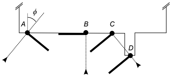
Fig. 2. Contact configurations. The contact points are indicated by circles. By convention, references to left and right are relative to the approach line in the direction from \hat{p}_i into the part, and positive \phi is clockwise. By definition, if \phi_j > 0 , the gripper jaw’s right edge must be on the approach line, and if \phi_j < 0 , the gripper jaw’s left edge must be on the approach line. If \phi_j = 0 , we define the approach line to be the gripper jaw’s right edge. Configuration A shows an approach angle of -40^\circ , which implies a gripper to the right of the approach line. Configuration B shows an approach angle of 0^\circ , which by convention has a gripper to the left of the approach line. Configurations C and D show an approach angle of 40^\circ , which implies a gripper to the left of the approach line. Additionally, if configuration C was a nominal contact configuration g , the actual contact configuration g' would be configuration D.
