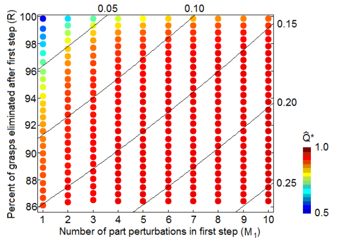
Fig. 14. Tradeoff in worst-case quality (color) and execution time (lines) over parameter combinations. The color of each dot indicates the average worst-case \hat{Q}^* for the parameter values. For example, the point in the upper left represents M_1 = 1 and 99.85% of grasps eliminated (i.e., R = 0.0015 ), meaning after one part perturbation is tested, one grasp is selected from the successful grasps on that perturbation, and tested on the remainder of the perturbations. This point has a \hat{Q}^* of 0.577. Contours of \hat{\eta} between 0.05 and 0.25 are shown. The parameter values at any point along a contour require the same number of grasp evaluations.
