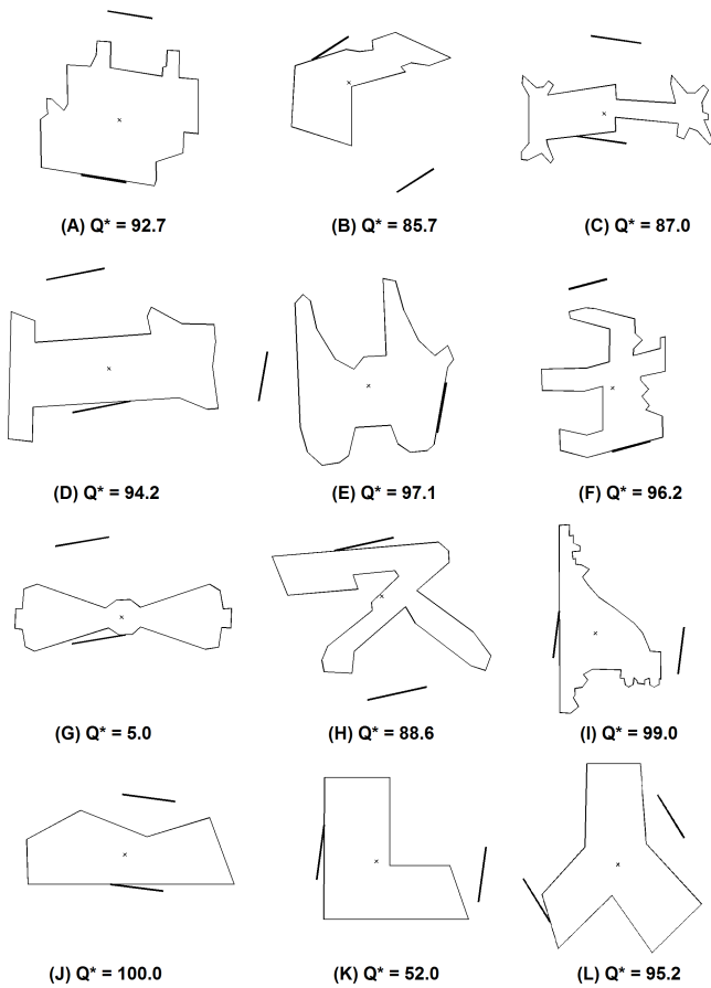
Fig. 6. The test set of brackets. The g^* grasps for parameters d_C = 0 , \rho = 1.5 , and |\Phi| = 5 are depicted. The grasps are indicated with the pushing jaw in contact with the part, and the closing jaw opposite it away from the part. “Whisker diagrams” showing detailed results for Parts A and B can be seen in Figures 7 and 8, respectively. Part G has a problematic shape for the algorithm. The size of the gripper prevents it from contacting the edges very near the center of mass. The long, straight edges are outside the inverse friction cone of the center of mass, meaning a contact on them will slip. The ends of the part are narrow and consist of several different edges, which, under perturbation, can prevent conservative-slip pushes or force closure from being achieved. Part K is also problematic. As shown in Table I, a 100% successful grasp is possible, but is only found with a very dense grasp set. With the grasp set used here, the best grasp only has a Q -value of 52.0. This is because the shape of part means grippers that are in good position relative to the center of mass are in areas that are very sensitive for force closure.
