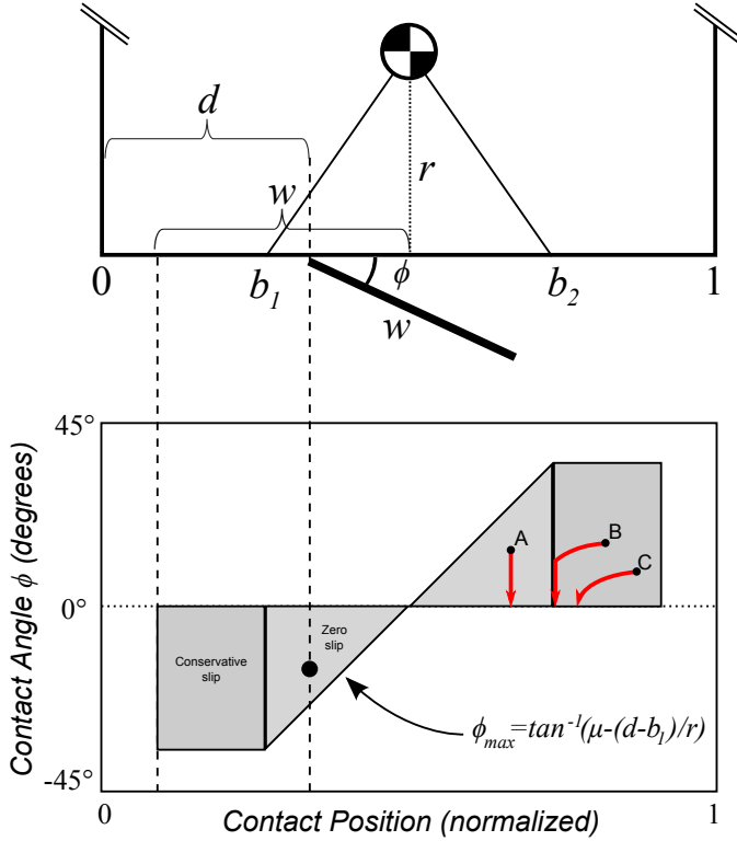
Fig. 4. Configuration space for fast analysis. The upper half of the figure shows a gripper of width w contacting the part at position d with (negative) contact angle \phi = 30^\circ , inverse friction cone bounds b_1 and b_2 and perpendicular distance r from the center of mass. Contact with this edge of the part results in the configuration space shown below it; the shaded area is the region where a conservative-slip push occurs. The red lines in the lower region show the configuration-space path for a zero-slip push (A) and possible paths for two conservative-slip pushes (B and C) from initial contact, but cannot increase in contact angle or move away from the center of mass. If the path intersects the zero-slip region, it follows a zero-slip path, shown by path B.
