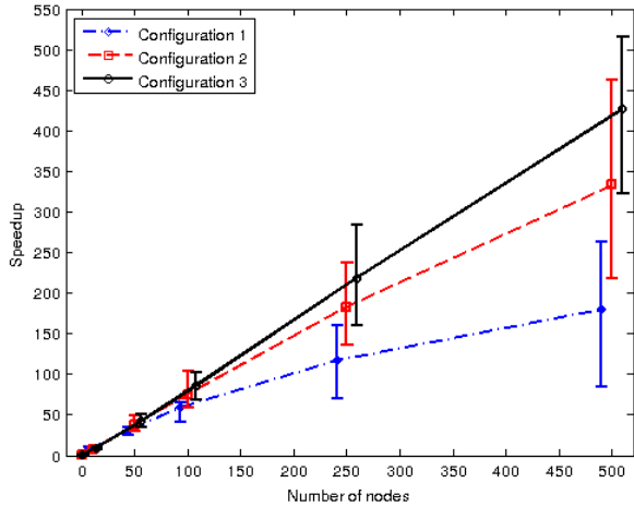
Fig. 15. Average MATLAB runtime speedup vs. number of nodes. The average, minimum, and maximum are shown for 1, 10, 50, 100, 250, and 500 nodes. The highest speedup is 515\times , for Part A with Configuration 3.
