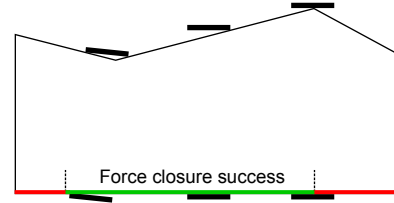
Fig. 5. Force closure modes. Slip closure is shown by the gripper pair on the right; friction closure is shown by the gripper pair in the middle; and convex vertex closure is shown on the right.
